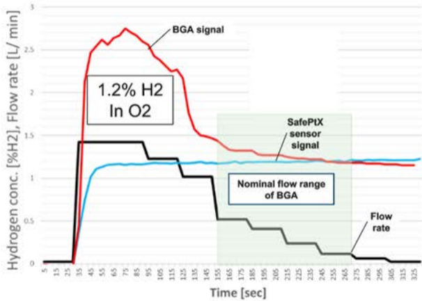
Varying flow rate of 1.2% H 2 in O 2
