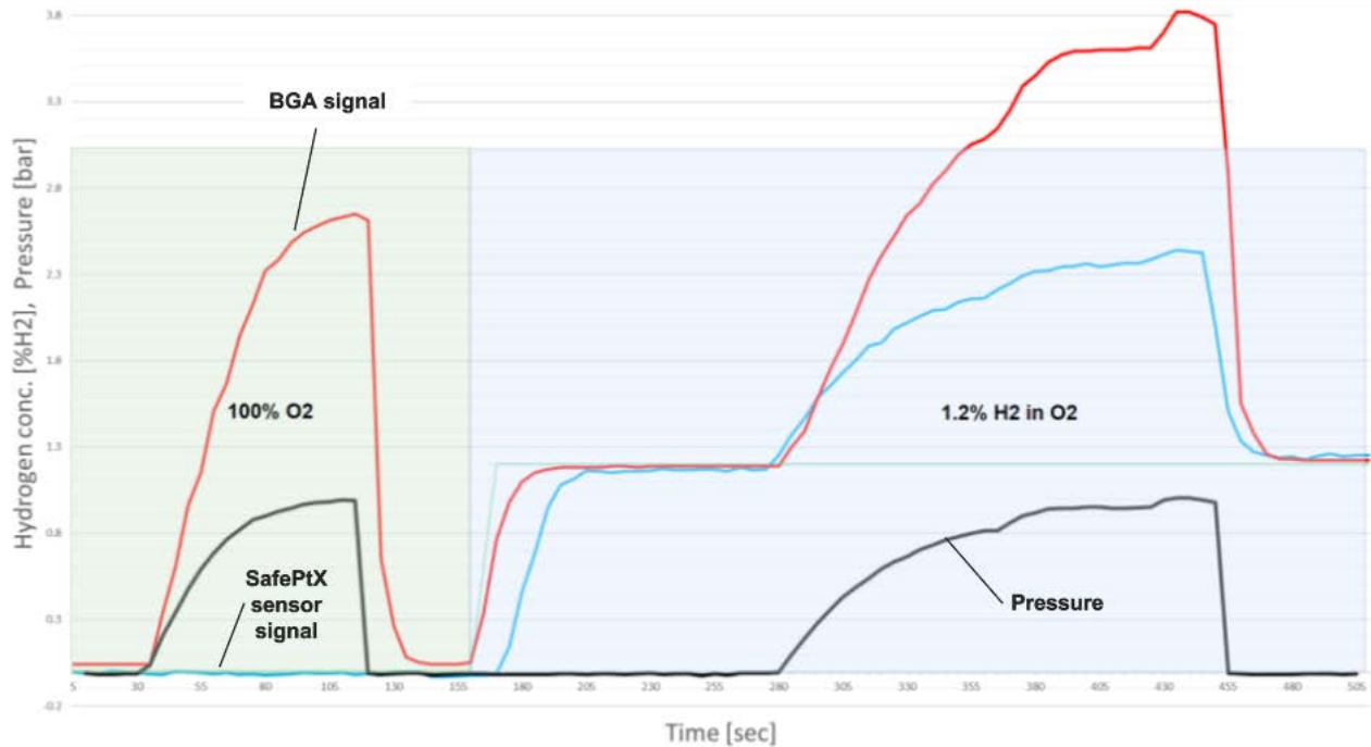
Pressure vs %H2 measured
