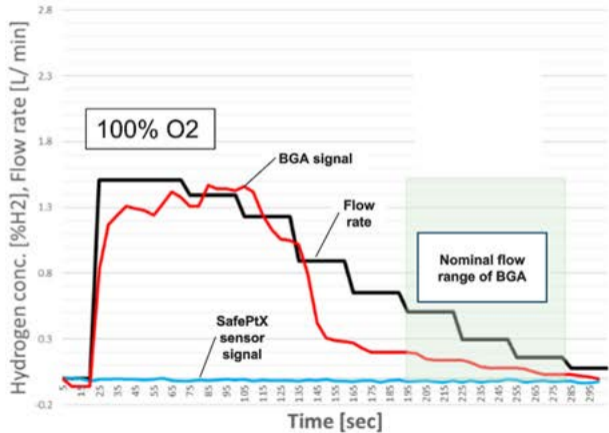
Varying flow rate of pure O 2
