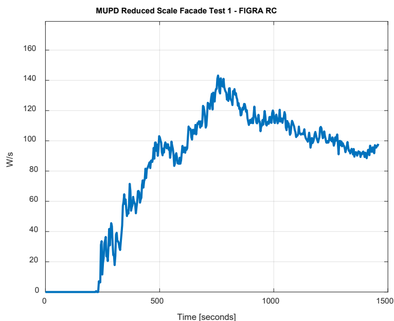
Figur 13. FIGRA Fire Growth Rate
