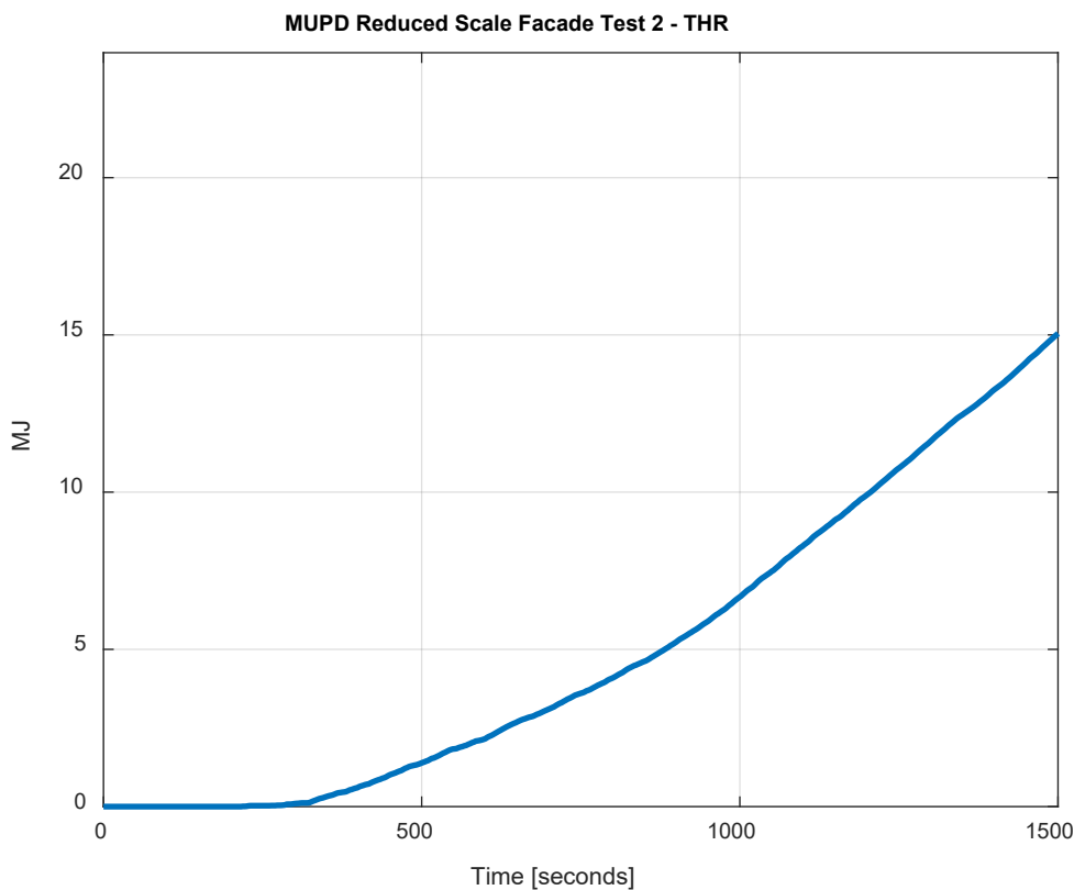
Figur 16 Total Heat release Rate
